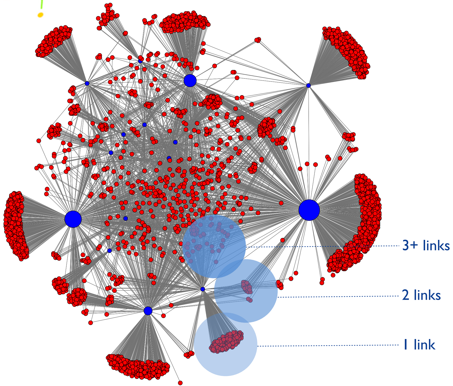
Force-directed graph with 1+ indegree links (seeds in blue, other nodes in red). Fruchterman-Reingold algorithm.
